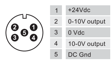
5 pins M12 connector (View toward sensor pins)
