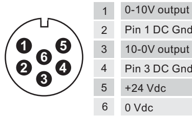
D60 connector (View toward sensor pins)
